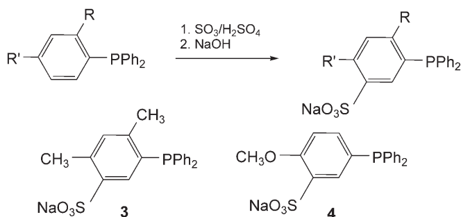
Scheme 1. Recently developed derivatives of TPPMS.
