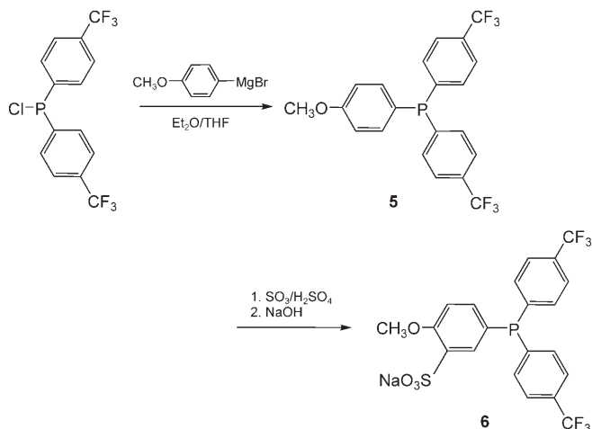
Scheme 2. Synthesis of 6 , a \pi -acceptor TPPMS derivative.
